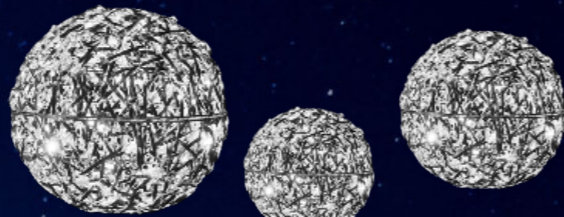
7 Orbitals 3D
